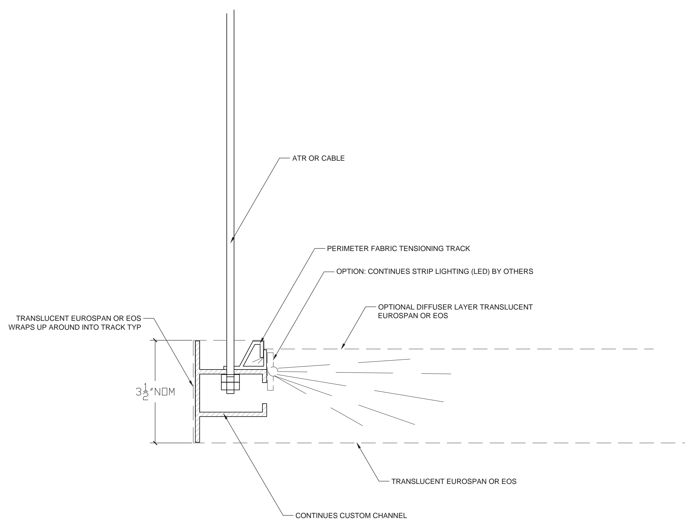
A TRANSLUCENT EUROSPAN® OR EOS CEILING CLOUD - OPTIONAL LIGHTING TRANS HALF SCALE
